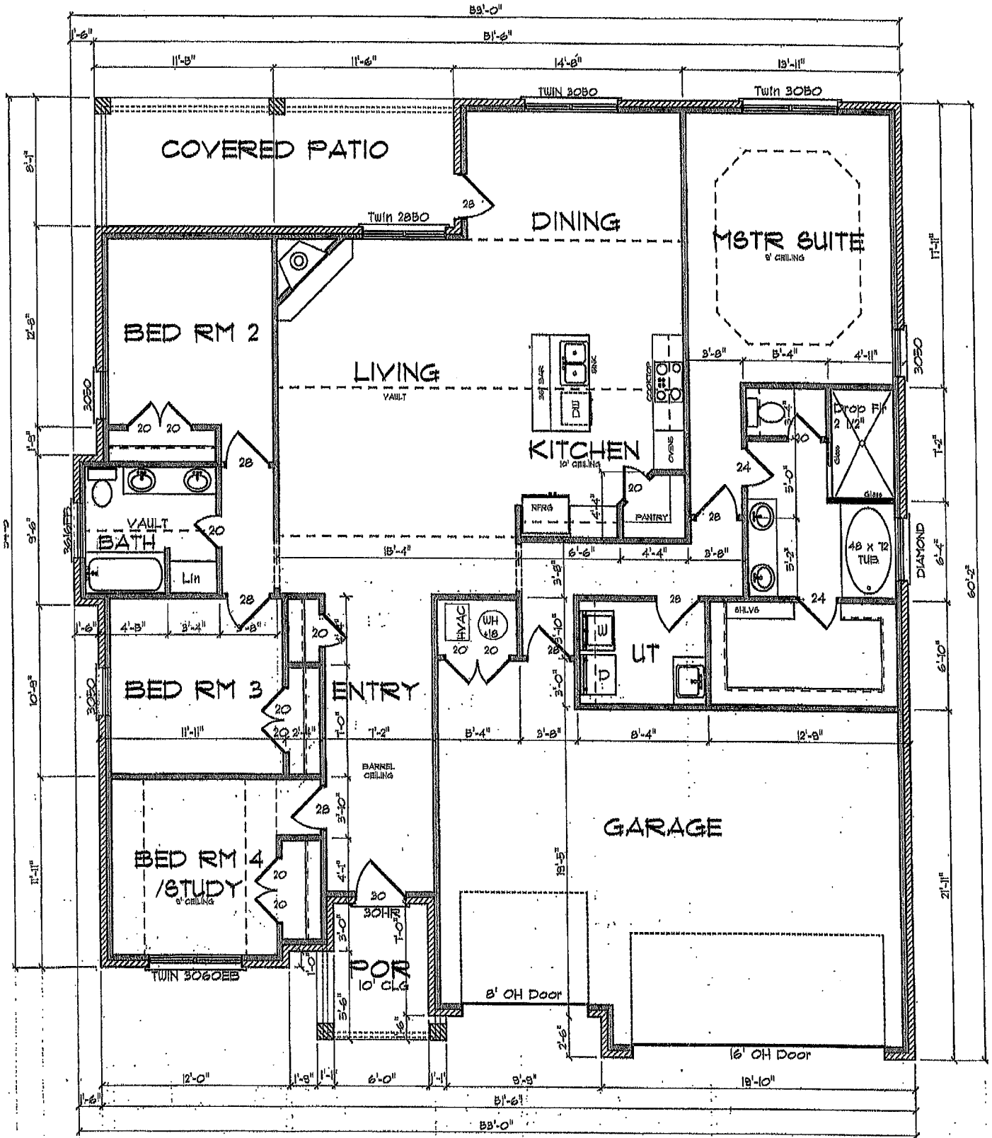
FLOOR PLAN SCALE: 1/4" = 1'-0"
